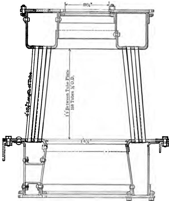
FIG. 164.—The Thornycroft Steam Wagon Boiler.
